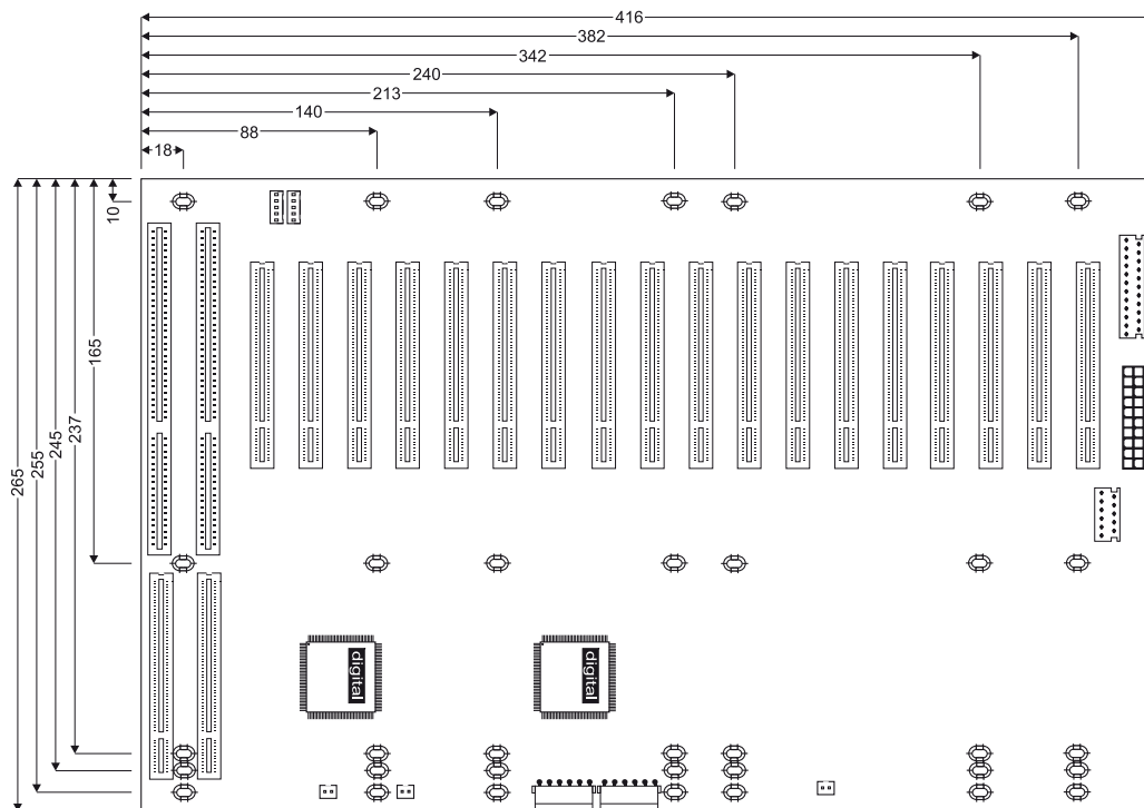
Layout
